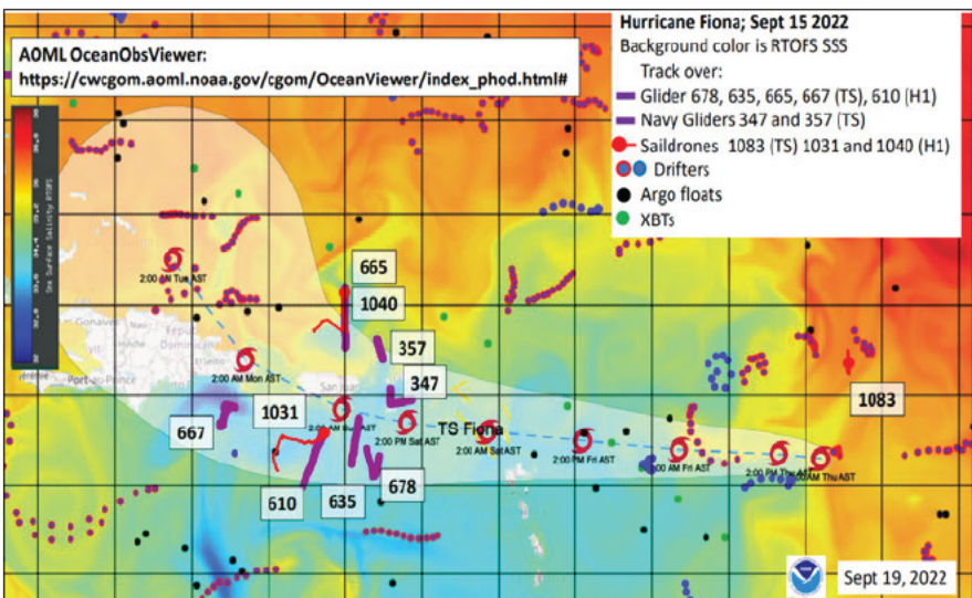
Map of the Atlantic basin showing the location of ocean-observing instruments and track of Fiona in September 2022.
