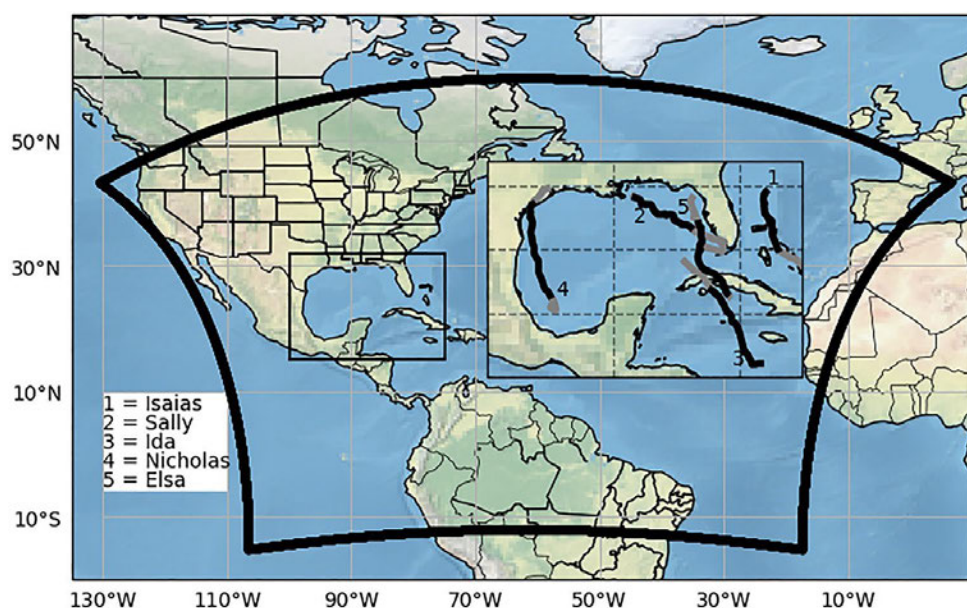
Model domain outlined by a thick black line with two inset panels. The small panel shows the regions traversed by Isaias, Sally, Ida, Nicholas, and Elsa in the Gulf of Mexico, northwest Caribbean Sea, and southwest Atlantic. The large panel shows the analyzed track periods (black track lines) and unanalyzed simulation periods (gray lines) for the five tropical cyclones (from Alvey and Hazelton, 2022).
