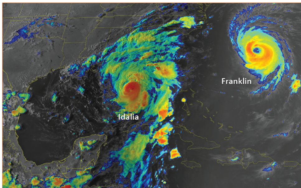
NOAA GOES-East satellite image of Hurricane Idalia approaching the west coast of Florida and Hurricane Franklin churning in the western Atlantic on August 24, 2023.
