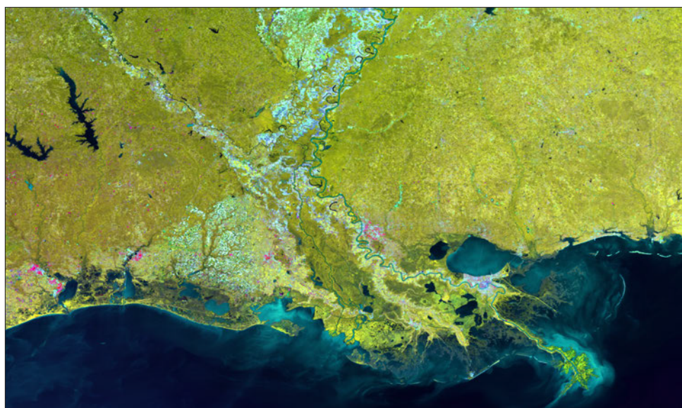
Satellite image of the Mississippi River Delta on October 8, 2016 showing plumes of sediment and phytoplankton along the Gulf of Mexico coast. Image credit: NOAA-NESDIS.
