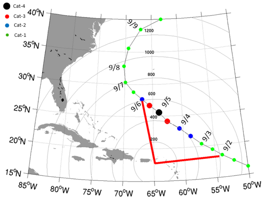
Figure OC-1: Storm track with locations plotted every 12 hours. Range rings are 200 n mi relative to the forward operating base at St. Croix, USVI (STX/TISX), and the red line delineates storm locations within 600 n mi of STX. In this example, the storm center remains within 600 n mi for 4 days.
