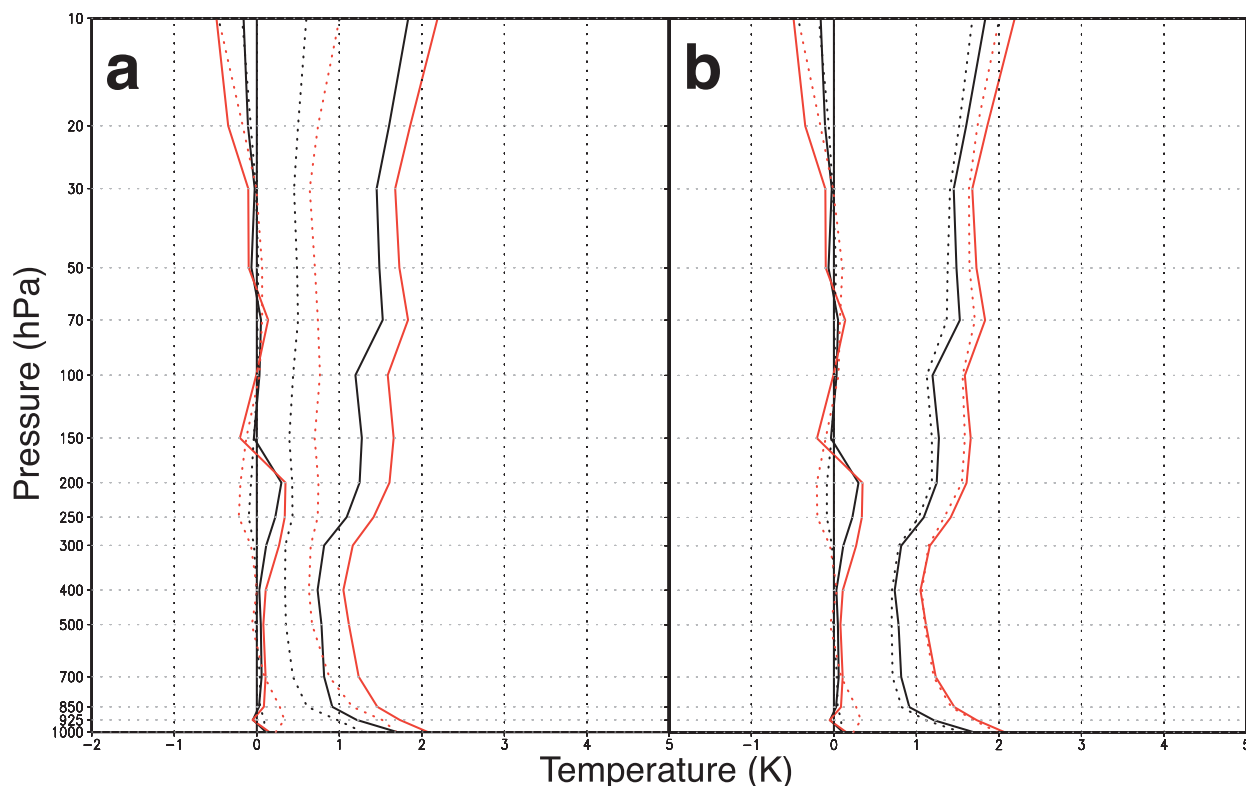
FIG. 4. Global mean and RMS differences for temperature innovations ( O - B , plotted in red) and analysis departures [observations minus analysis ( O - A ), plotted in black] for the period 0000 UTC 16–0000 UTC 22 May 2005. Solid lines are results for the OSE and dotted lines are results for the OSSE. The OSE results are the same in both panels. The OSSE results are for (a) perfect simulated observations (i.e., with no added errors) and (b) simulated observations with calibrated errors added. [Graphic created by J. Woollen, NOAA/Environmental Modeling Center (EMC).]
