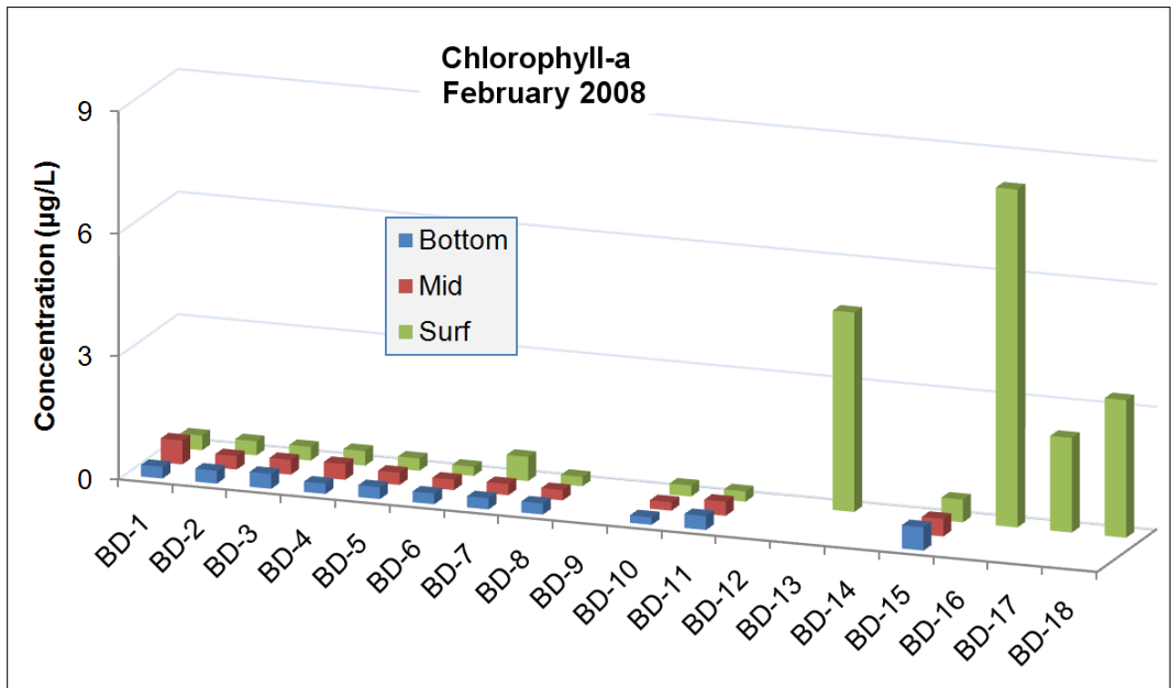
Figure 52: February 2008 chlorophyll-a concentrations for the Boynton-Delray water quality monitoring stations.
