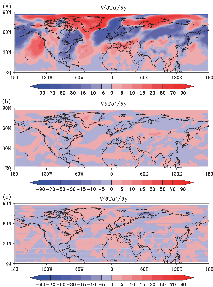
Figure 4. The contributions of the meridional temperature advection difference in Figure 3(b) by (a) the advection of mean temperature gradient by anomalous wind ( -V'\partial\bar{T}_a/\partial y ), (b) the advection of anomalous temperature gradient by mean wind ( -\bar{V}\partial T'_a/\partial y ) and (c) the nonlinear advection ( -V'\partial T'_a/\partial y ). The unit is 10^{-4}^{\circ}\text{C/s} .
