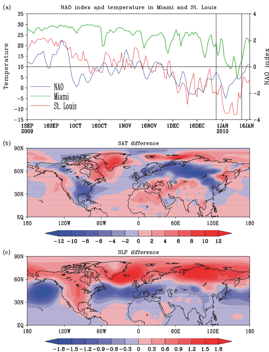
Figure 2. (a) Daily temperatures (°C) in Miami and St Louis and daily NAO index from 1 September 2009 to 18 January 2010. (b) SAT difference (°C) between the period of 28 December 2009 and 13 January 2010 (D28–J13) and the same time period of previous 60 years. (c) SLP difference (hPa) between the period of D28–J13 and the same time period of previous 60 years. Two vertical lines in (a) represent the weeks of D28–J13.
