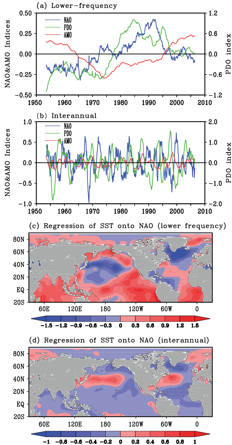
Figure 5. (a) The lower-frequency (7-year running mean) NAO, PDO and AMO (°C) indices. (b) The interannual NAO, PDO and AMO indices. (c) Regression (°C/NAO) of monthly SST onto the lower-frequency NAO index. (d) Regression (°C/NAO) of monthly SST onto the interannual NAO index. The interannual index is calculated as the difference between the 1-year running mean index and the 7-year running mean index.
