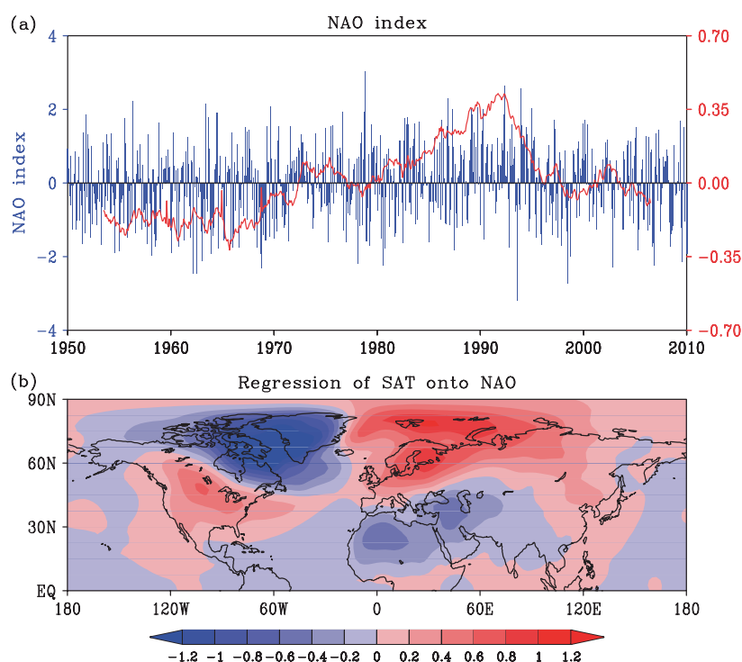
Figure 1. (a) Monthly NAO index from 1950 to 2009. (b) Regression ( ^\circ\text{C}/\text{NAO} ) of monthly surface air temperature onto the monthly NAO index. The red line in (a) is the 7-year running mean NAO index.
