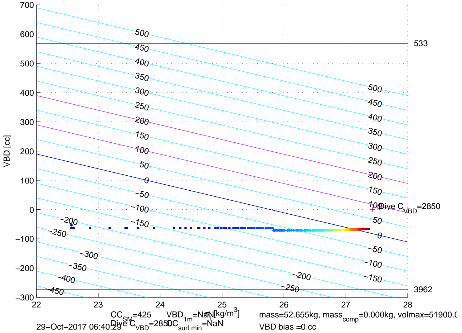
p6350752: SG635 Mission 7 Jul 2017 29-Oct-2017 05:48:05Z – buoyancy contoured
