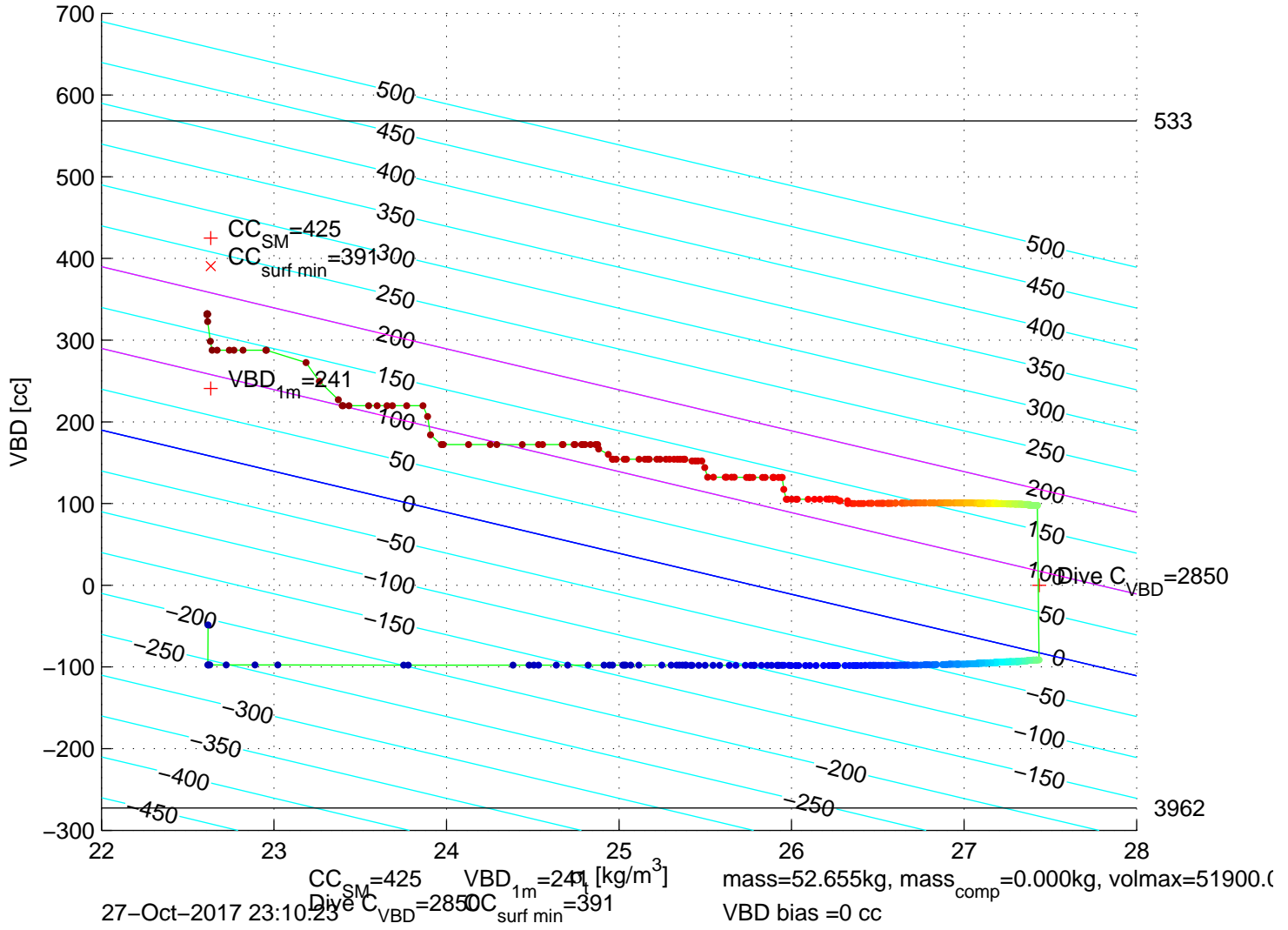
p6350745: SG635 Mission 7 Jul 2017 27-Oct-2017 22:32:56Z – buoyancy contoured
