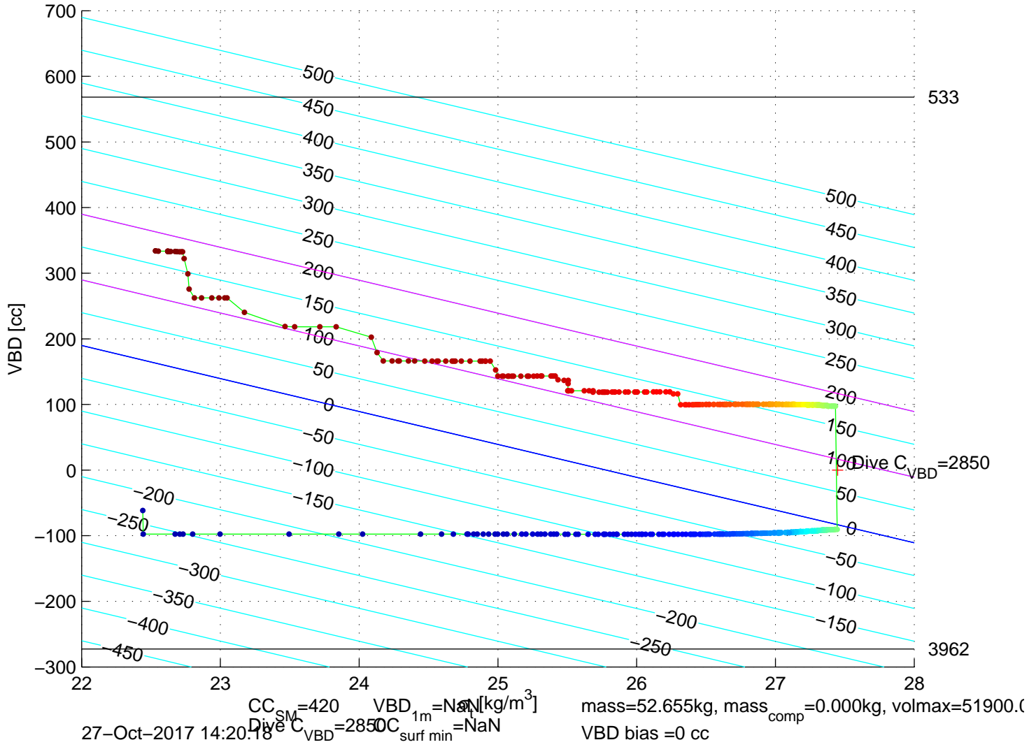
p6350743: SG635 Mission 7 Jul 2017 27-Oct-2017 13:32:42Z – buoyancy contoured
