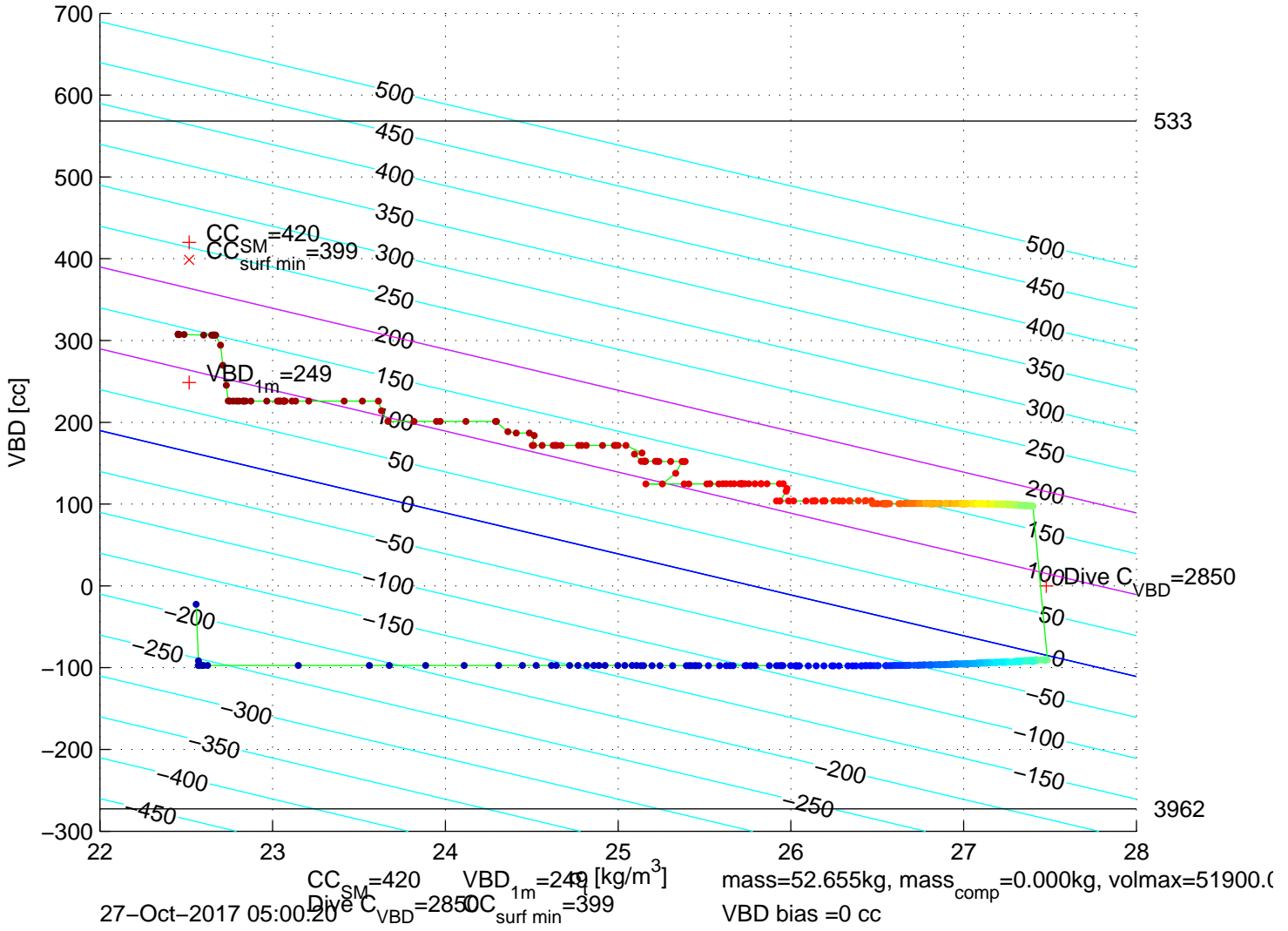
p6350741: SG635 Mission 7 Jul 2017 27-Oct-2017 04:21:23Z – buoyancy contoured
