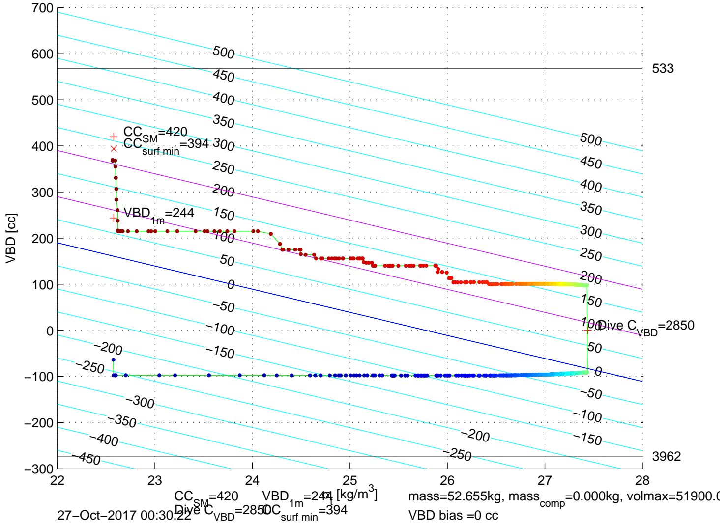
p6350740: SG635 Mission 7 Jul 2017 26-Oct-2017 23:42:24Z – buoyancy contoured
