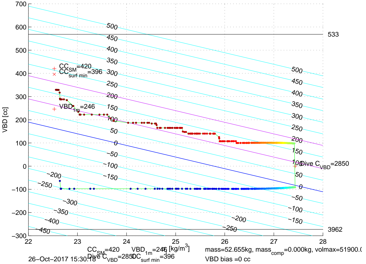
p6350738: SG635 Mission 7 Jul 2017 26-Oct-2017 14:53:30Z – buoyancy contoured
