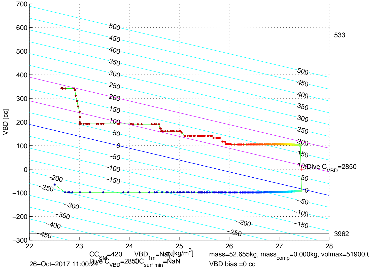
p6350737: SG635 Mission 7 Jul 2017 26-Oct-2017 10:18:11Z – buoyancy contoured
