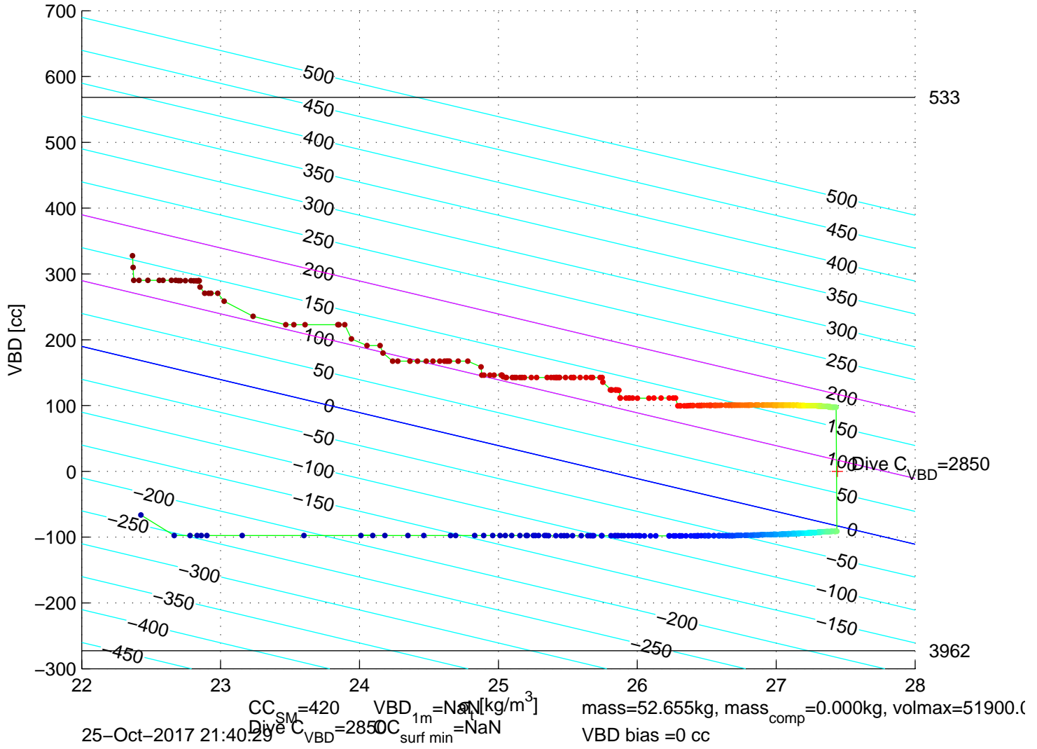
p6350734: SG635 Mission 7 Jul 2017 25-Oct-2017 20:58:04Z – buoyancy contoured
