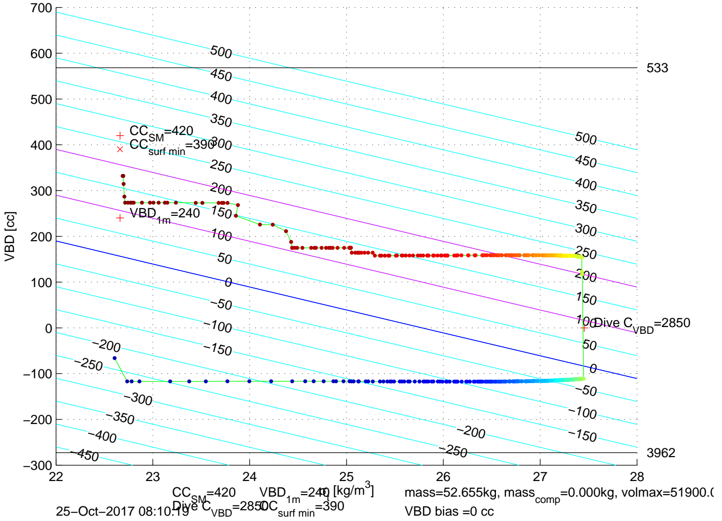
p6350731: SG635 Mission 7 Jul 2017 25-Oct-2017 08:08:32Z – buoyancy contoured
