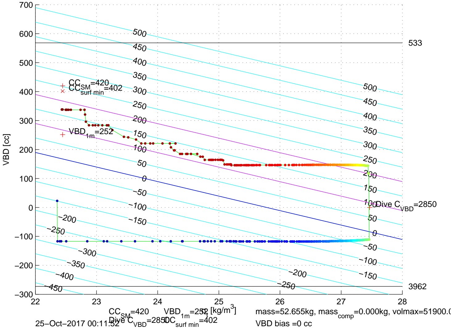
p6350729: SG635 Mission 7 Jul 2017 24-Oct-2017 23:57:03Z – buoyancy contoured
