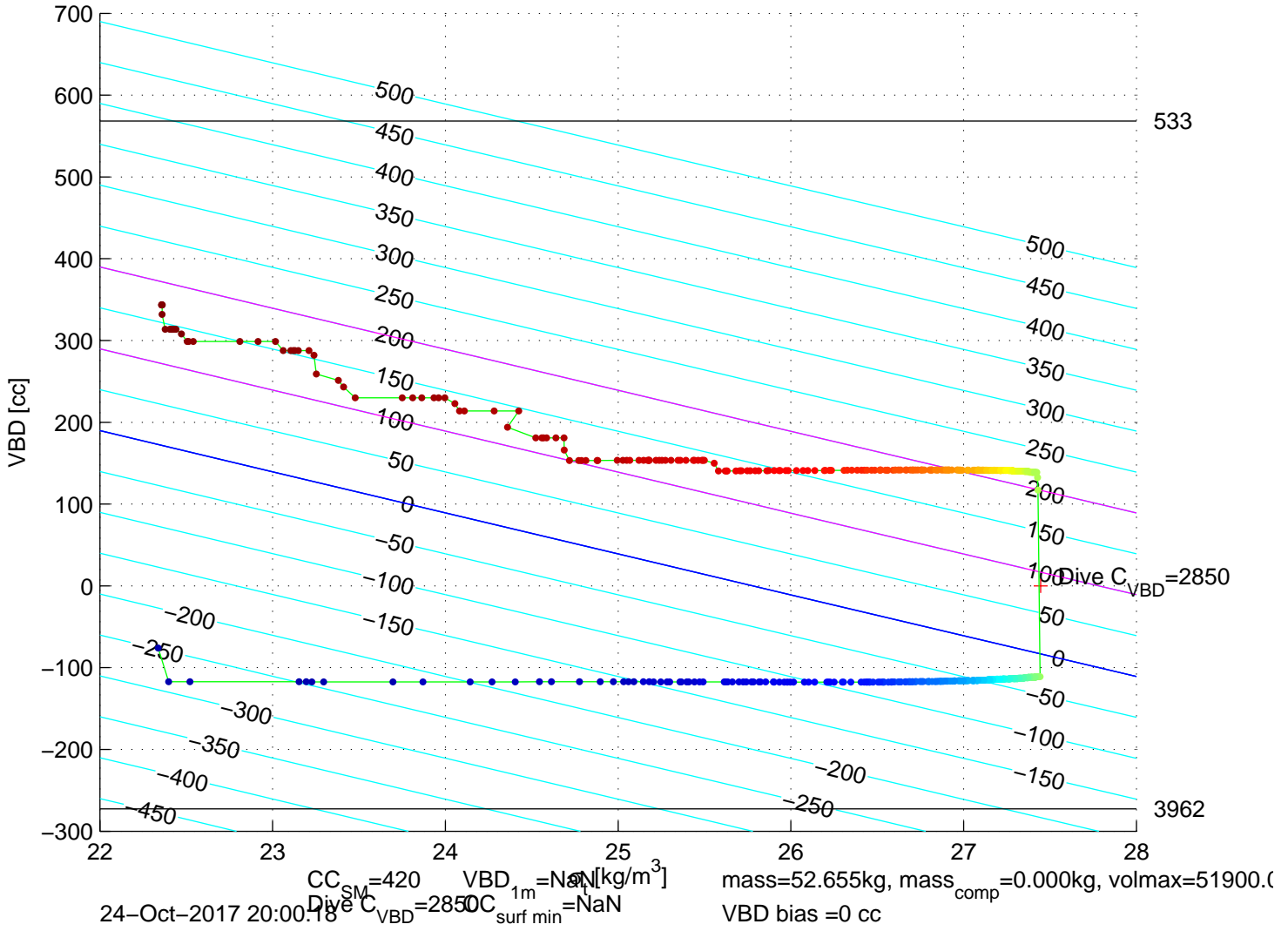
p6350728: SG635 Mission 7 Jul 2017 24-Oct-2017 19:49:28Z – buoyancy contoured
