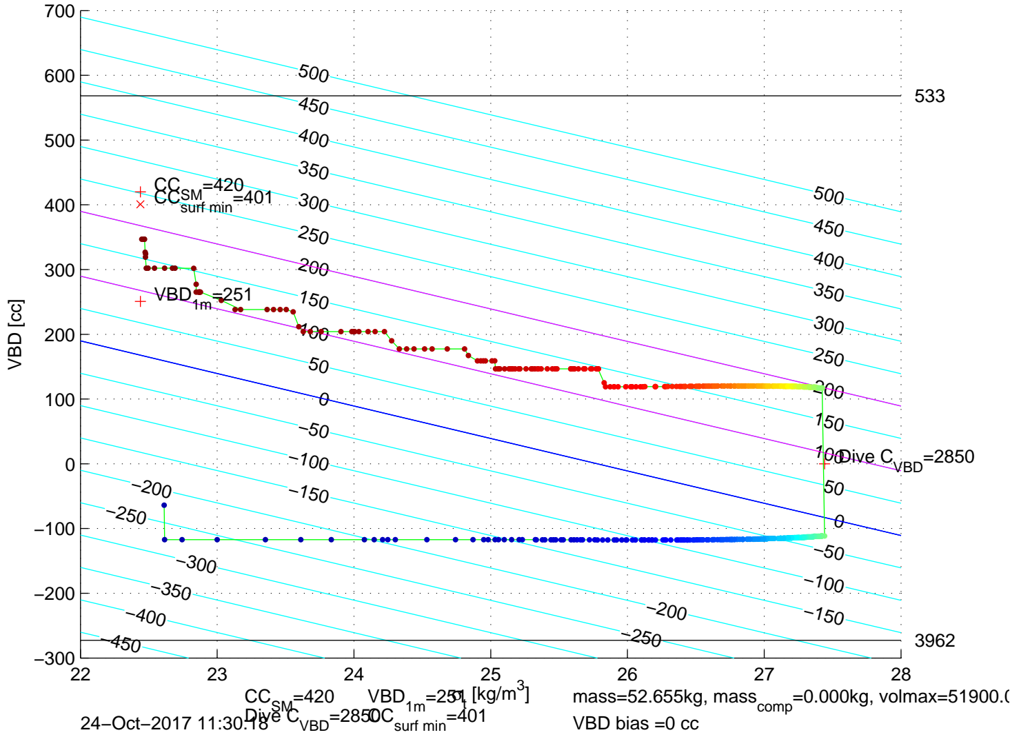
p6350726: SG635 Mission 7 Jul 2017 24-Oct-2017 11:06:18Z – buoyancy contoured
