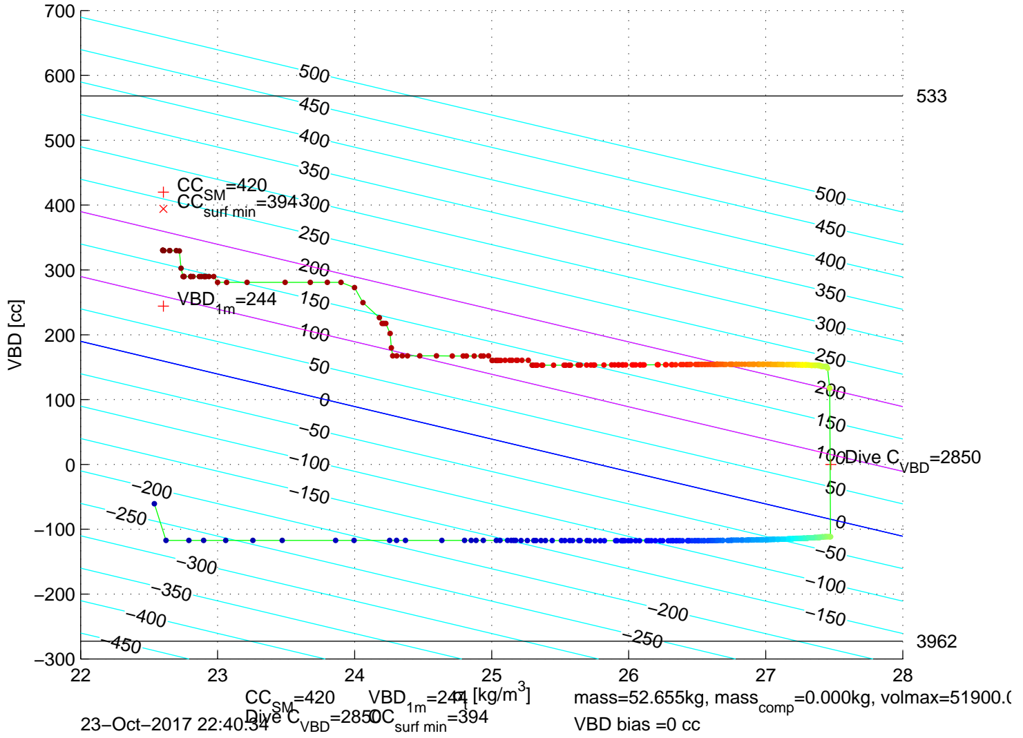
p6350723: SG635 Mission 7 Jul 2017 23–Oct–2017 22:30:03Z – buoyancy contoured
