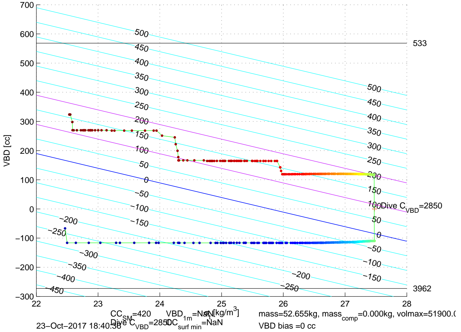
p6350722: SG635 Mission 7 Jul 2017 23-Oct-2017 18:09:09Z – buoyancy contoured
