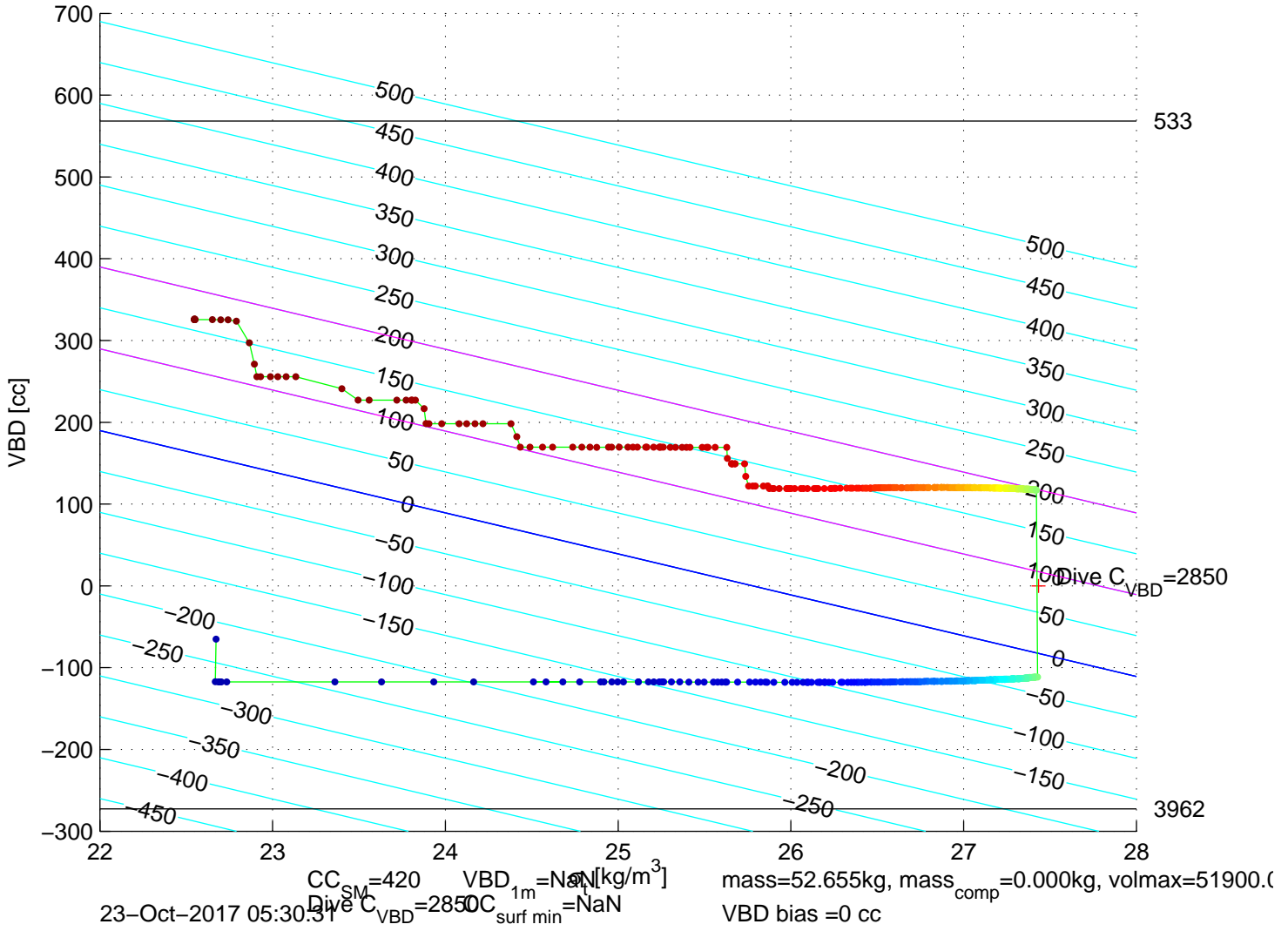
p6350719: SG635 Mission 7 Jul 2017 23-Oct-2017 05:00:08Z – buoyancy contoured
