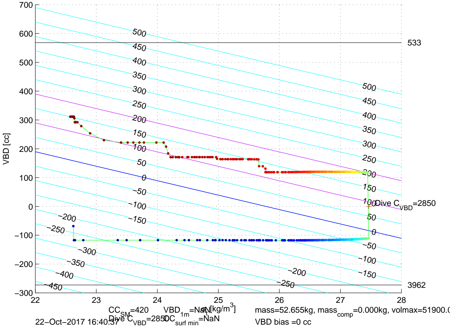
p6350716: SG635 Mission 7 Jul 2017 22-Oct-2017 16:13:58Z – buoyancy contoured
