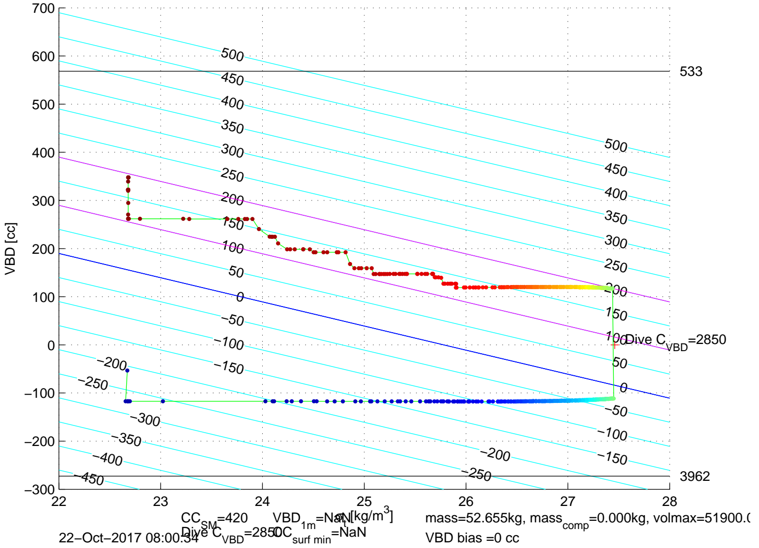
p6350714: SG635 Mission 7 Jul 2017 22-Oct-2017 07:37:33Z – buoyancy contoured
