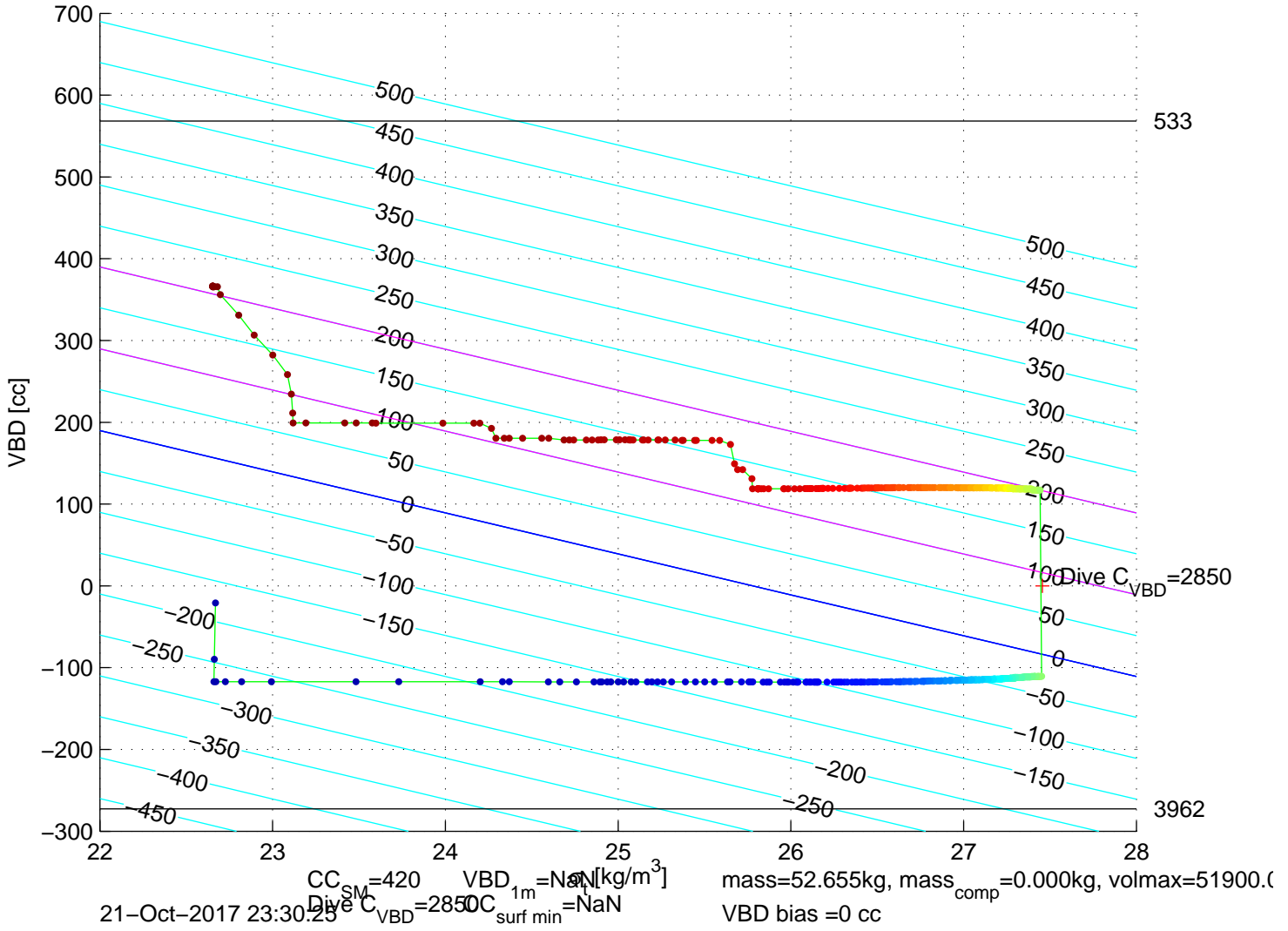
p6350712: SG635 Mission 7 Jul 2017 21-Oct-2017 23:04:51Z – buoyancy contoured
