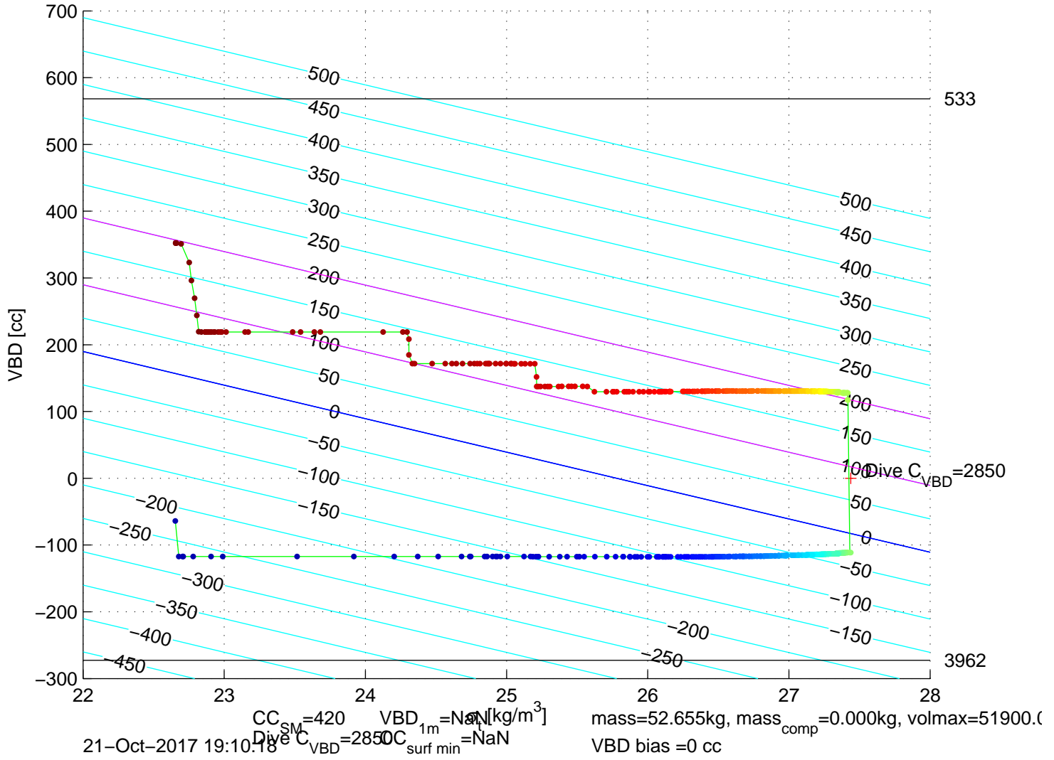
p6350711: SG635 Mission 7 Jul 2017 21-Oct-2017 18:42:58Z – buoyancy contoured
