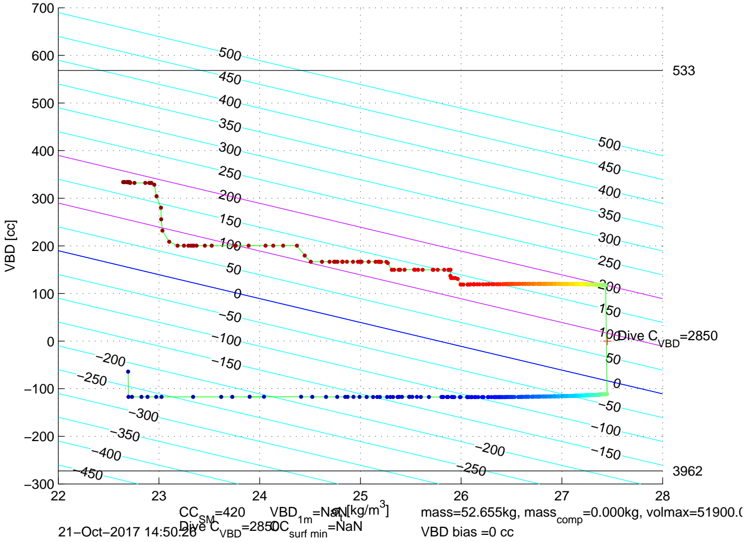
p6350710: SG635 Mission 7 Jul 2017 21-Oct-2017 14:24:12Z – buoyancy contoured
