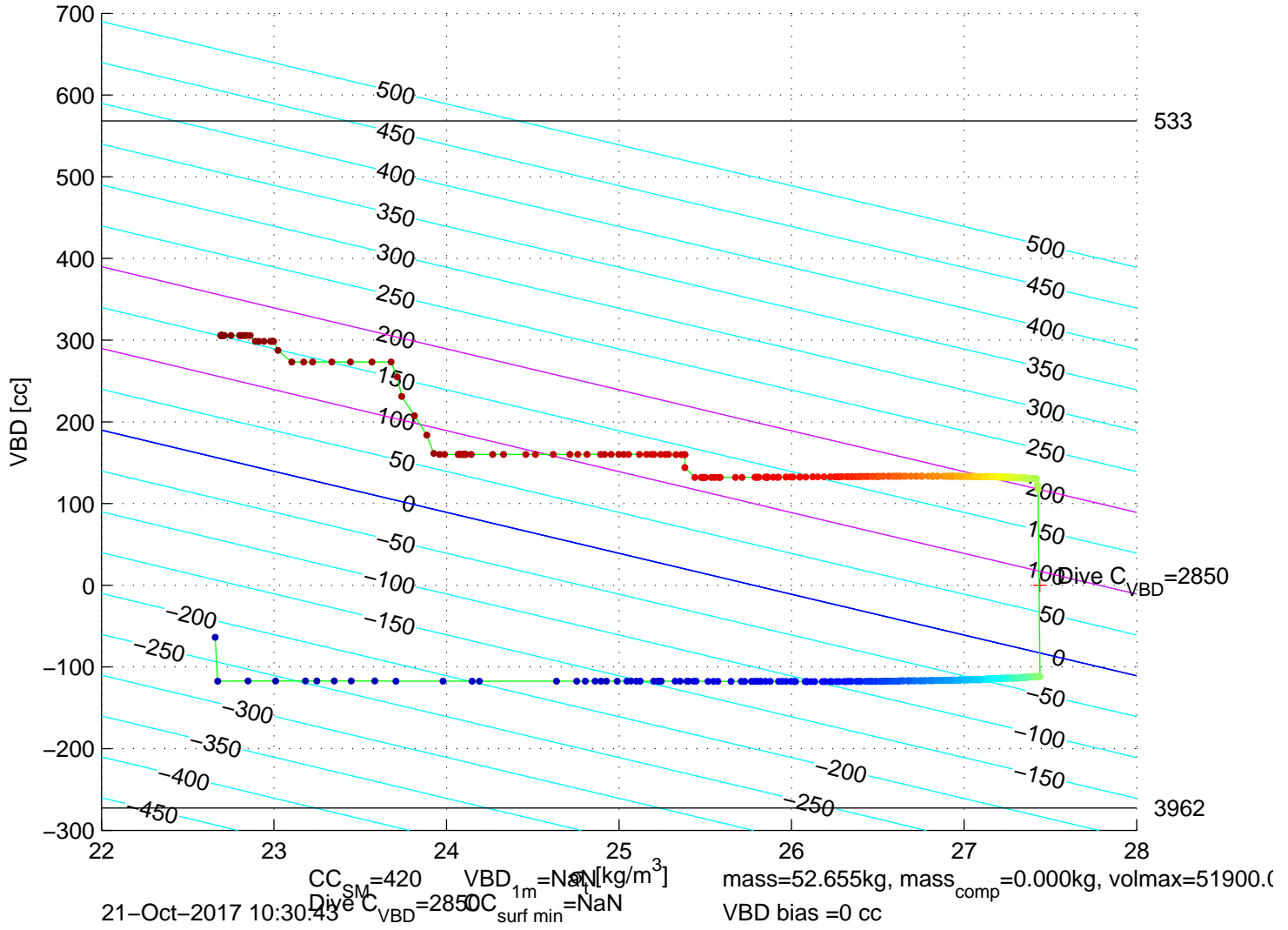
p6350709: SG635 Mission 7 Jul 2017 21-Oct-2017 10:12:27Z – buoyancy contoured
