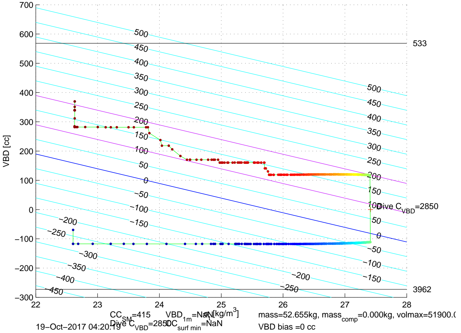
p6350696: SG635 Mission 7 Jul 2017 19–Oct–2017 03:49:29Z – buoyancy contoured
