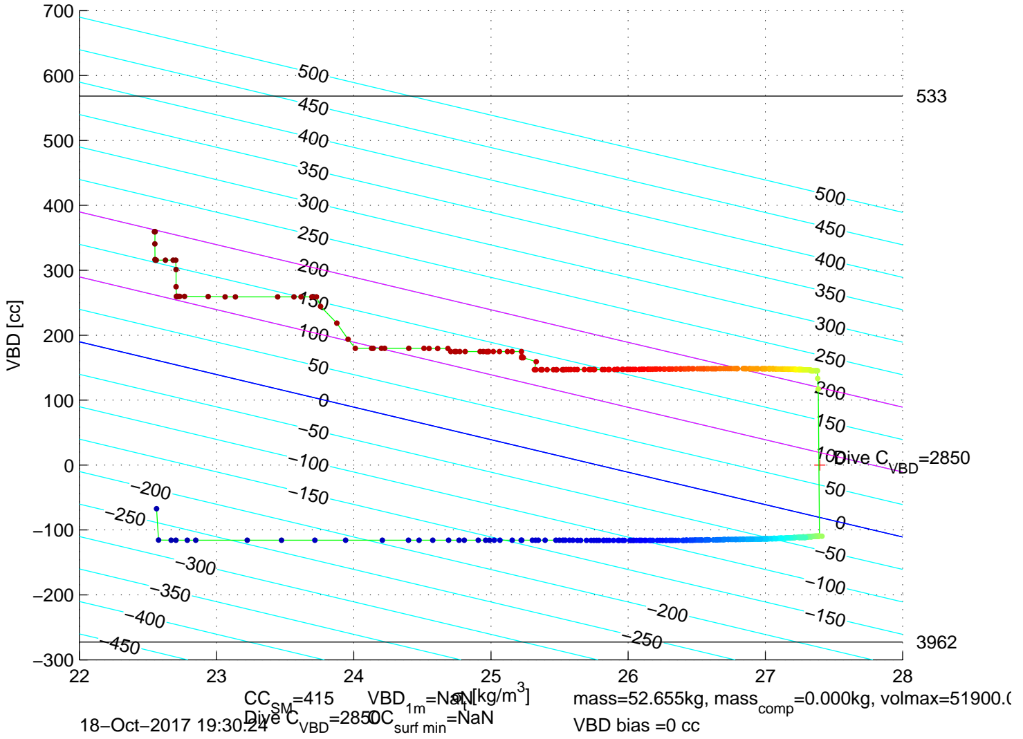
p6350694: SG635 Mission 7 Jul 2017 18-Oct-2017 19:15:15Z – buoyancy contoured
