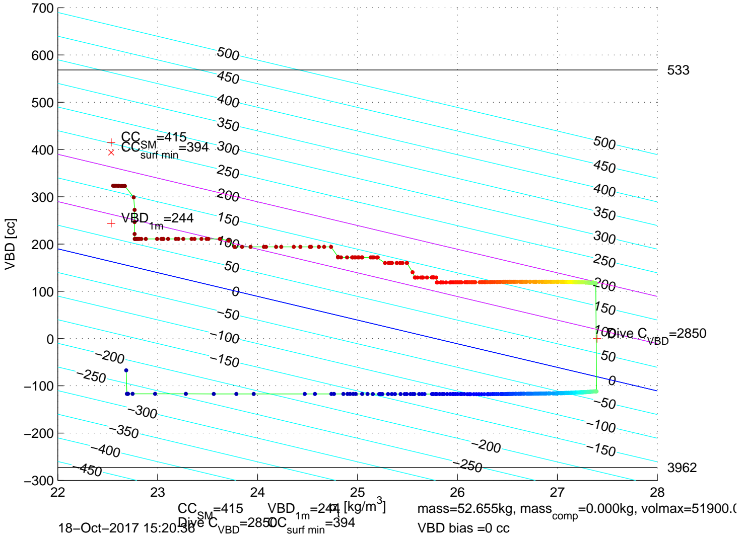
p6350693: SG635 Mission 7 Jul 2017 18-Oct-2017 14:54:11Z – buoyancy contoured
