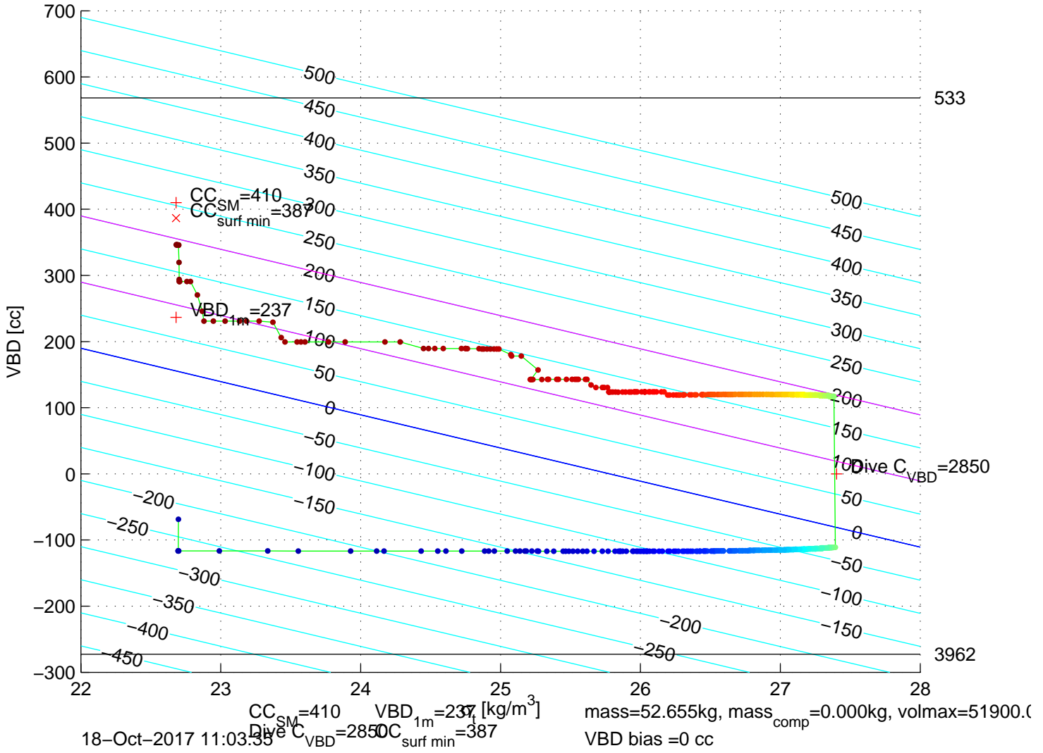
p6350692: SG635 Mission 7 Jul 2017 18-Oct-2017 10:31:20Z – buoyancy contoured
