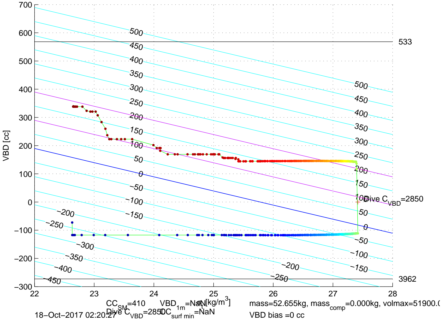
p6350690: SG635 Mission 7 Jul 2017 18-Oct-2017 02:13:24Z – buoyancy contoured
