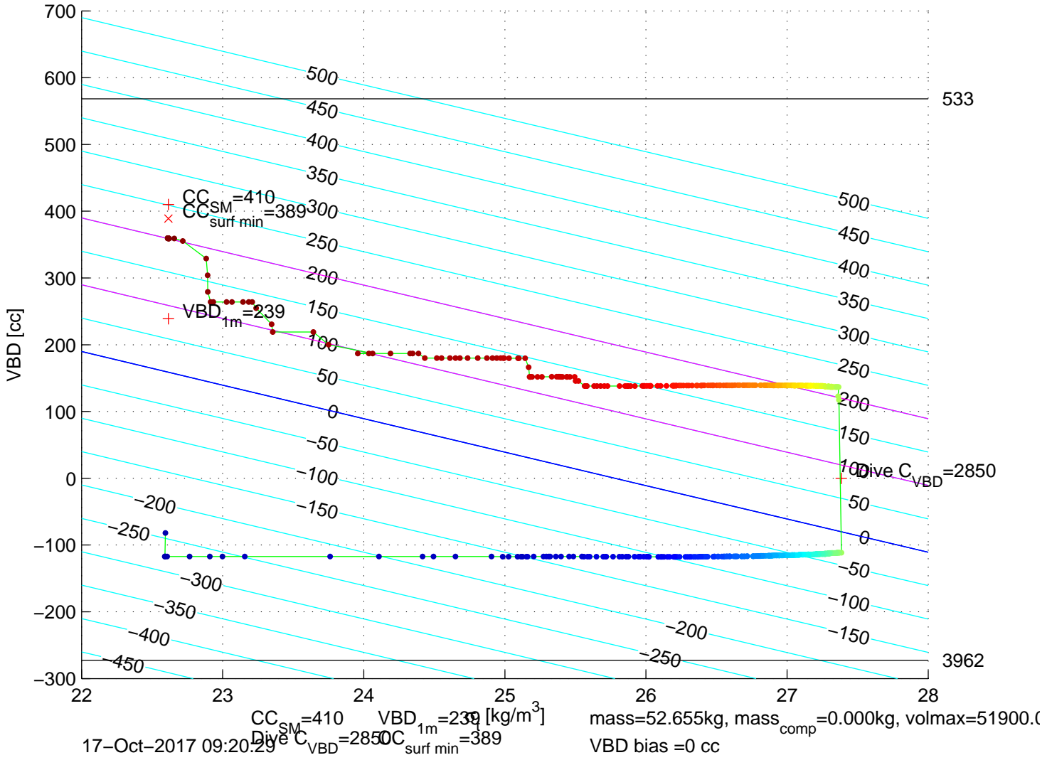
p6350686: SG635 Mission 7 Jul 2017 17-Oct-2017 09:08:42Z – buoyancy contoured
