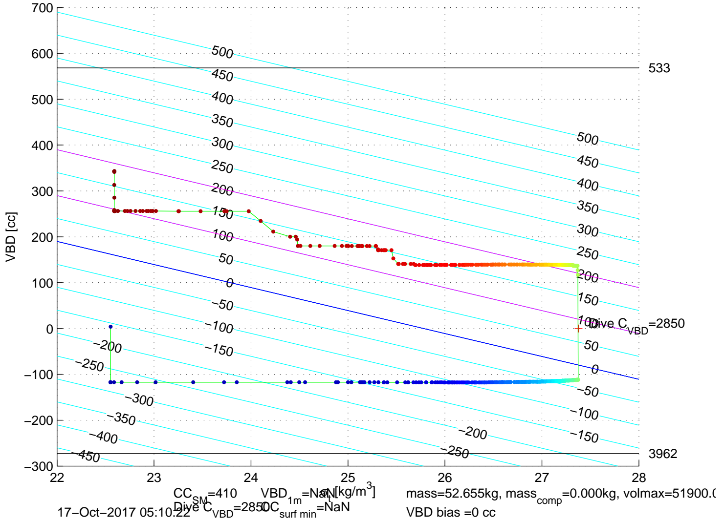
p6350685: SG635 Mission 7 Jul 2017 17-Oct-2017 04:57:34Z – buoyancy contoured
