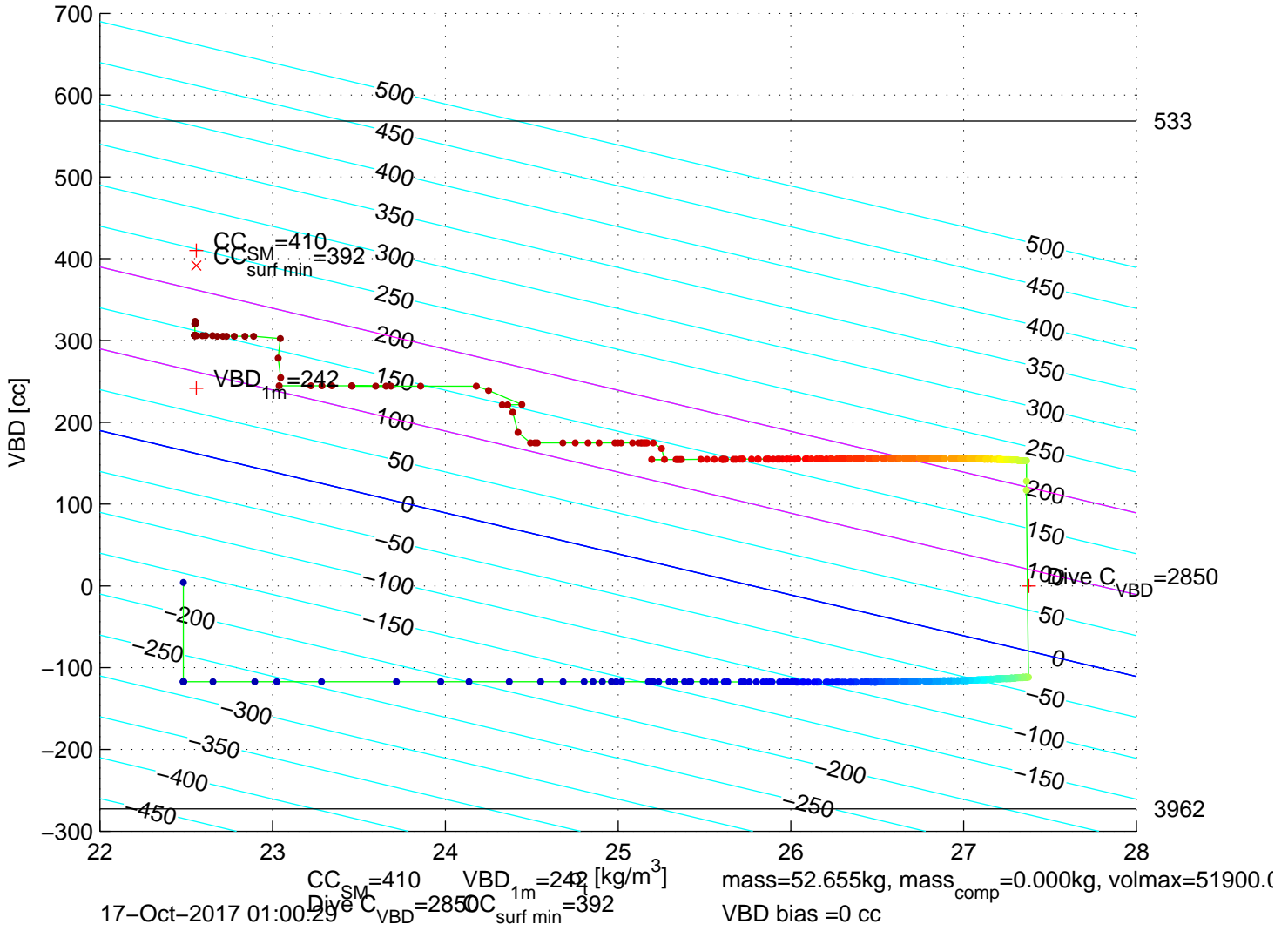
p6350684: SG635 Mission 7 Jul 2017 17-Oct-2017 00:55:50Z – buoyancy contoured
