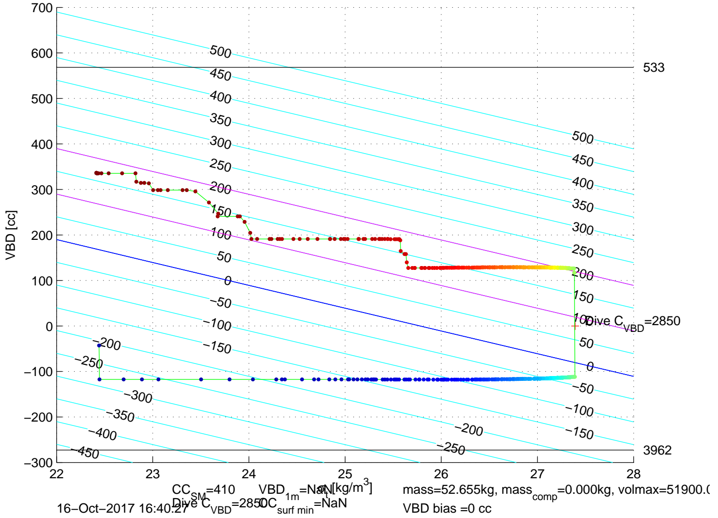
p6350682: SG635 Mission 7 Jul 2017 16-Oct-2017 16:17:17Z – buoyancy contoured
