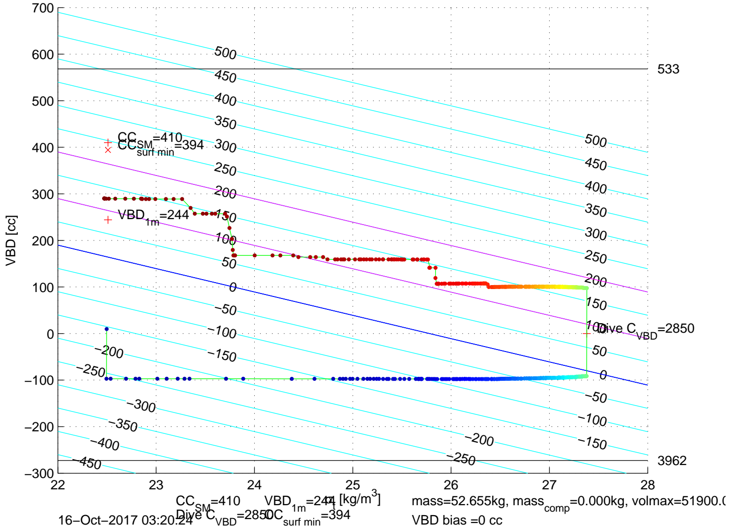
p6350679: SG635 Mission 7 Jul 2017 16–Oct–2017 02:35:16Z – buoyancy contoured
