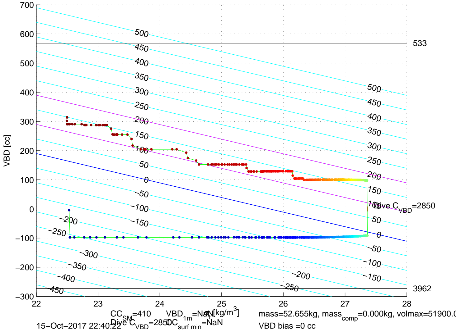
p6350678: SG635 Mission 7 Jul 2017 15–Oct–2017 21:58:41Z – buoyancy contoured
