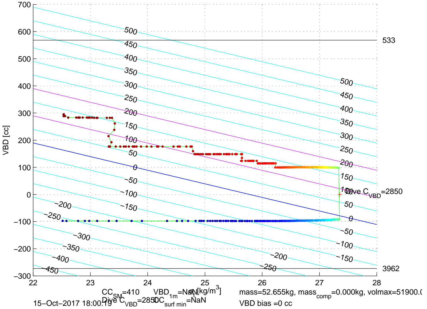
p6350677: SG635 Mission 7 Jul 2017 15–Oct–2017 17:17:38Z – buoyancy contoured
