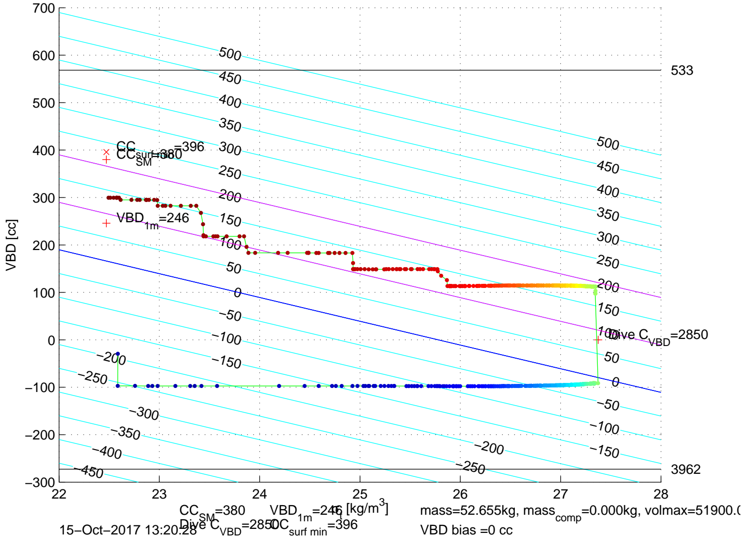
p6350676: SG635 Mission 7 Jul 2017 15–Oct–2017 12:44:45Z – buoyancy contoured
