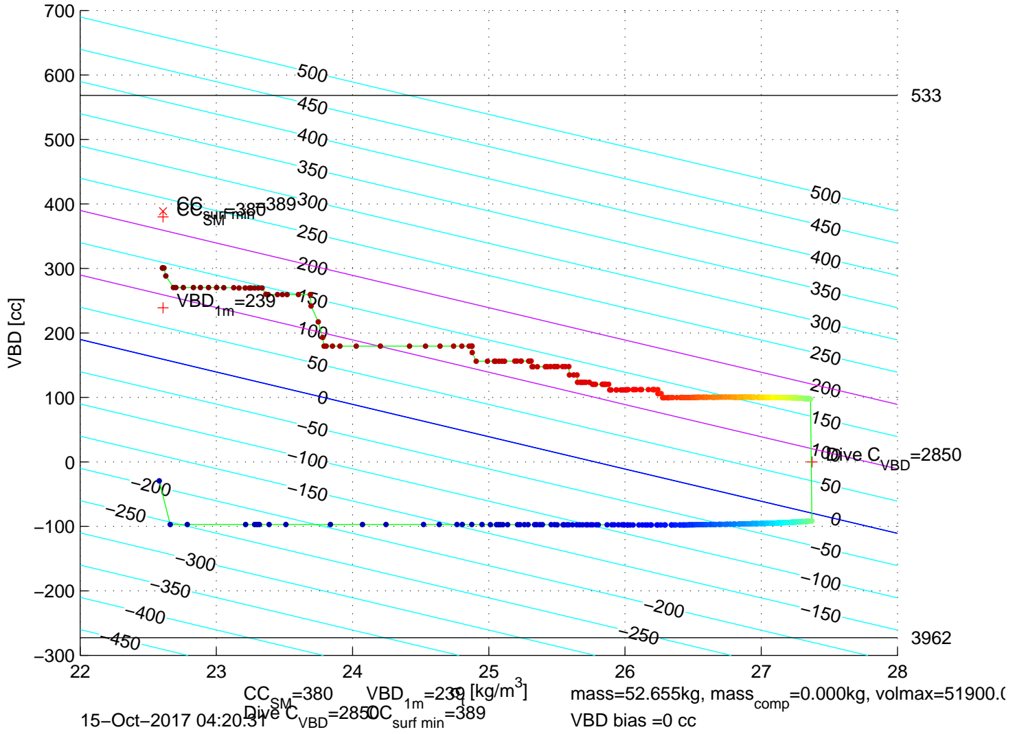
p6350674: SG635 Mission 7 Jul 2017 15–Oct–2017 03:35:08Z – buoyancy contoured
