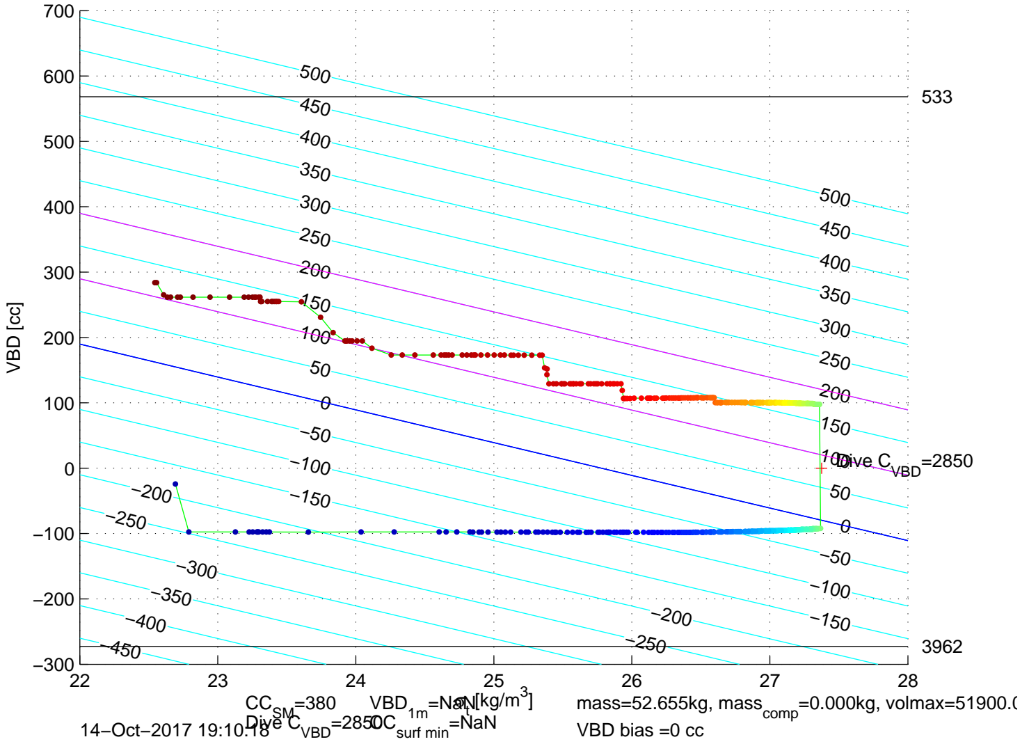
p6350672: SG635 Mission 7 Jul 2017 14–Oct–2017 18:33:04Z – buoyancy contoured
