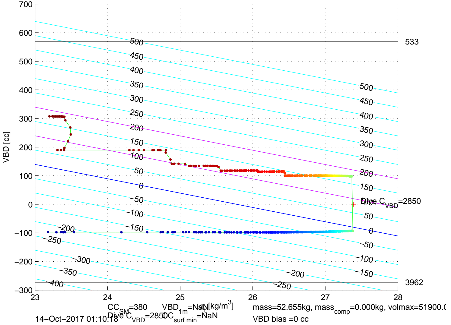
p6350668: SG635 Mission 7 Jul 2017 14-Oct-2017 00:35:26Z – buoyancy contoured
