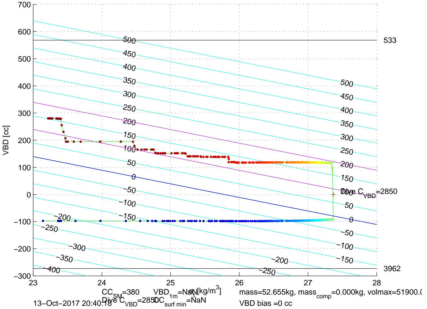
p6350667: SG635 Mission 7 Jul 2017 13–Oct–2017 20:16:03Z – buoyancy contoured
