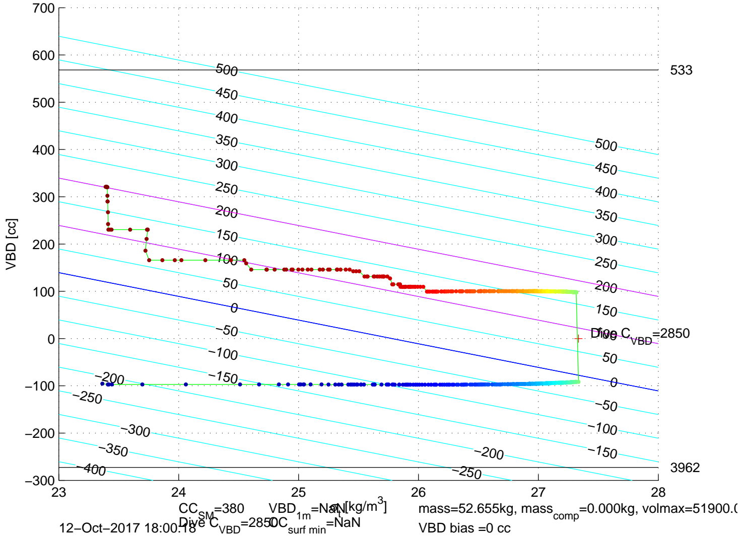
p6350661: SG635 Mission 7 Jul 2017 12–Oct–2017 17:19:24Z – buoyancy contoured
