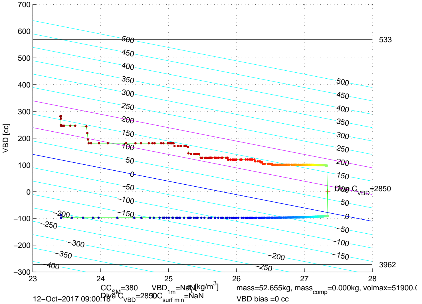
p6350659: SG635 Mission 7 Jul 2017 12–Oct–2017 08:18:21Z – buoyancy contoured
