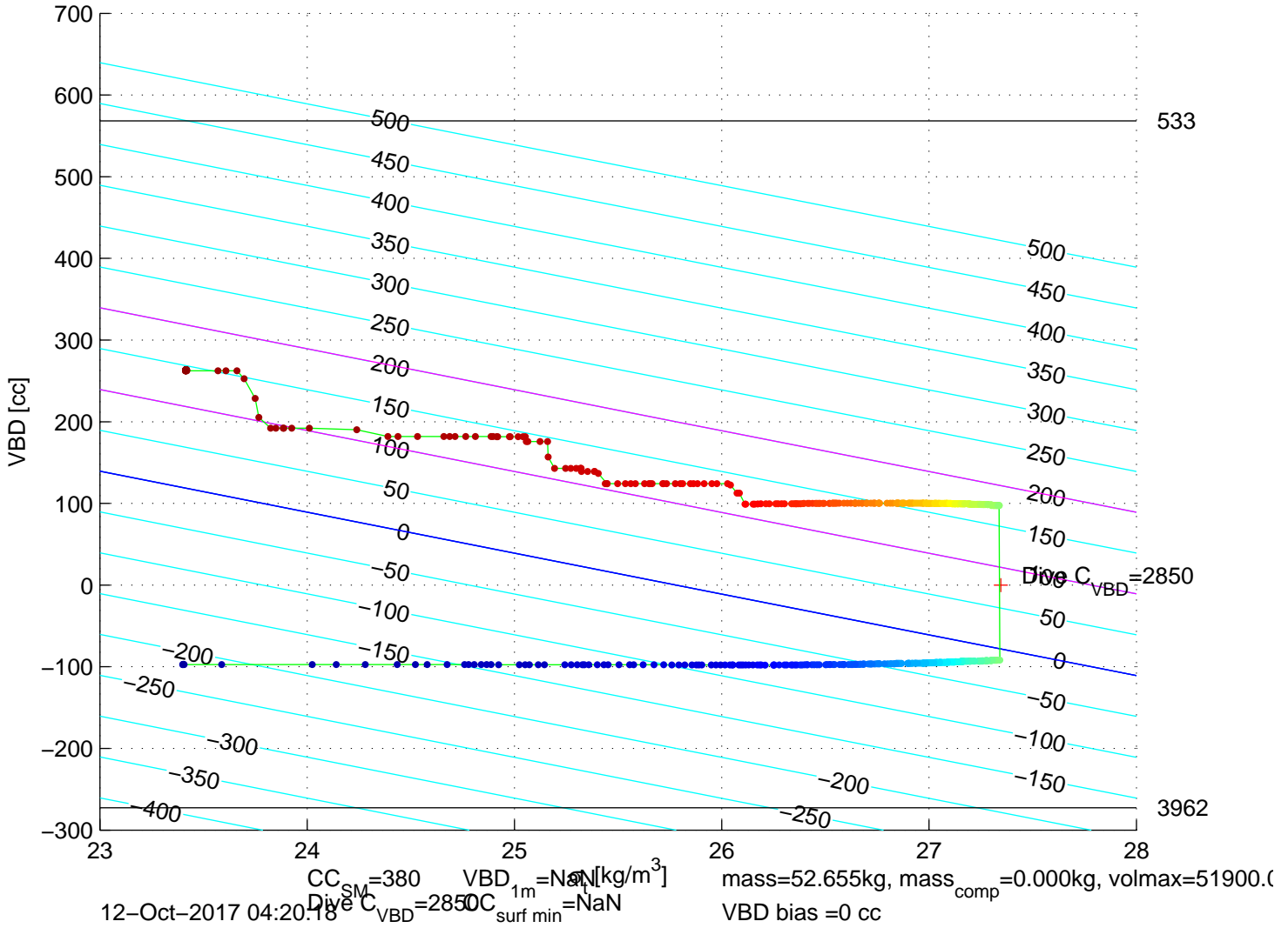
p6350658: SG635 Mission 7 Jul 2017 12-Oct-2017 03:42:27Z – buoyancy contoured
