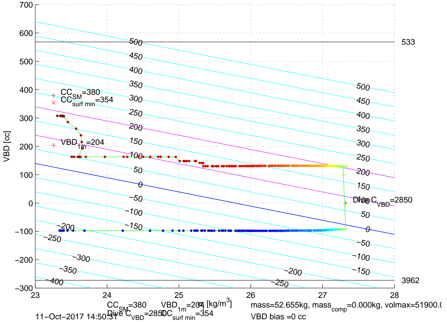
p6350655: SG635 Mission 7 Jul 2017 11-Oct-2017 14:27:49Z – buoyancy contoured
