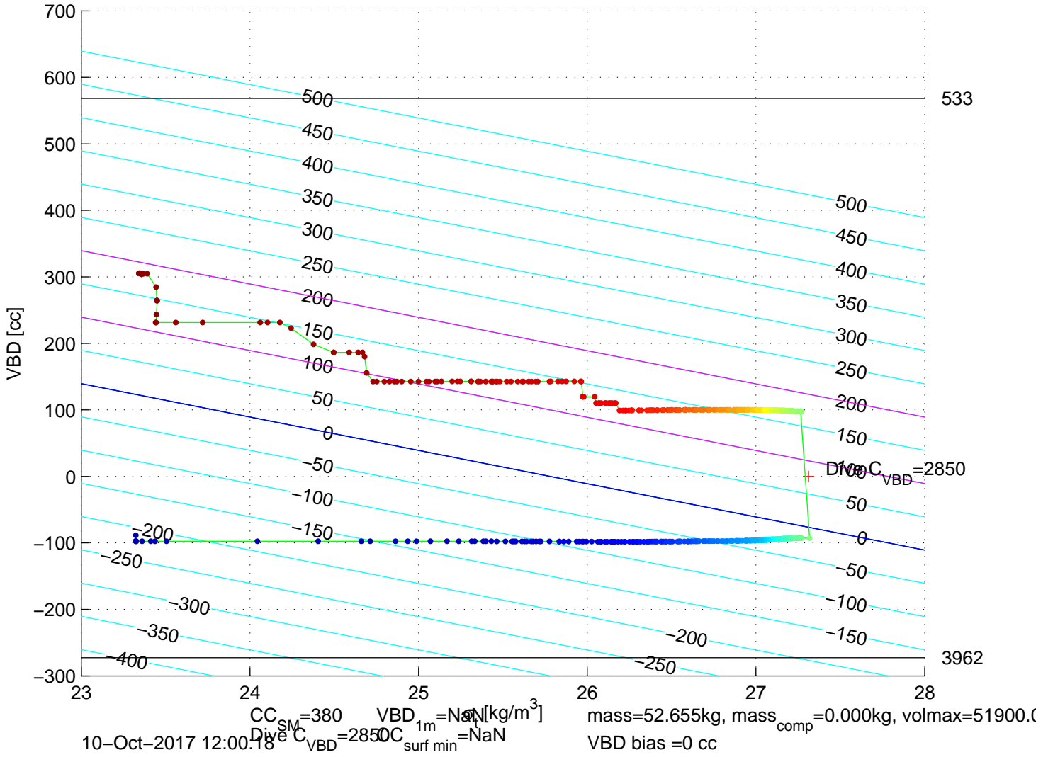
p6350649: SG635 Mission 7 Jul 2017 10–Oct–2017 11:12:40Z – buoyancy contoured
