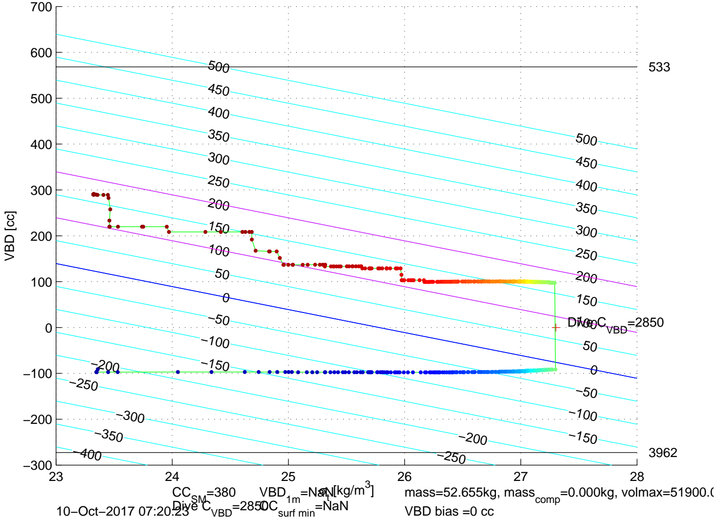
p6350648: SG635 Mission 7 Jul 2017 10–Oct–2017 06:42:40Z – buoyancy contoured
